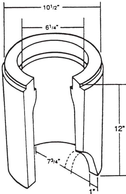
W1RVB Valve Box 40 lbs.
