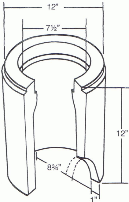
8VB Valve Box 48 lbs.
