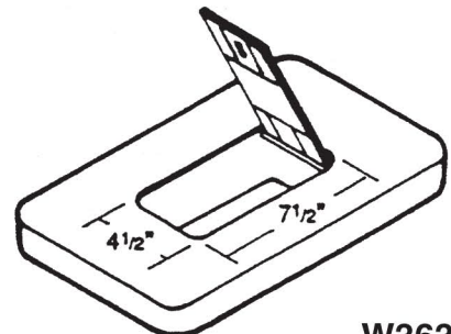
W363HL Concrete Cover Cast Iron Hinged Lid Frame 20 lbs.
